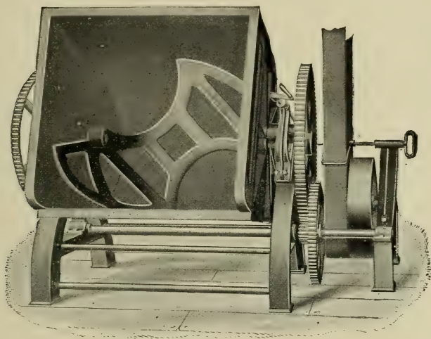
FIG. 116.—Mixer for Incorporating Large Percentages of Fillers in Asphalt.
